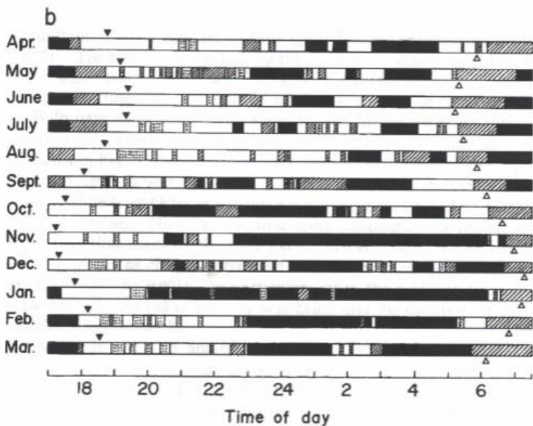
Fig. 6. Monthly changes in nocturnal activity for an adult male (a) and female (b) in captivity. Open, dotted, hatched and solid areas indicate movement or flapping, feeding, resting or self-grooming, and sleeping, respectively. ▼, sunset ; △, sunrise.
